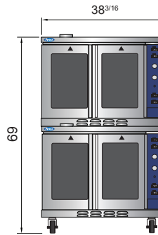
ATCO-513B-2
