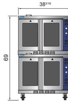
ATCO-513NB-2
